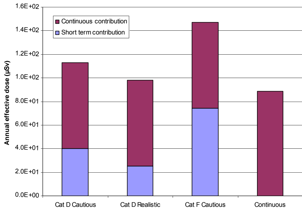
Figure 12 Case study 1 – Adult annual doses (µSv) at 1200 m from an AGR
