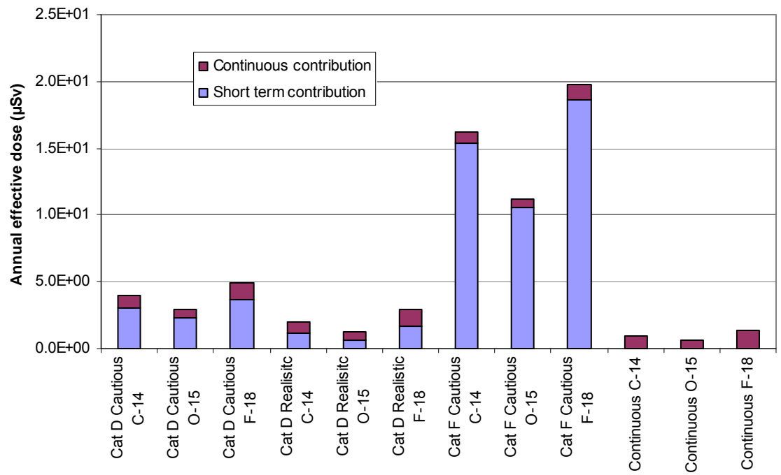
Figure 17 Case study 2 - Infant annual doses ( \mu\text{Sv} ) at 100 m from cyclotron
